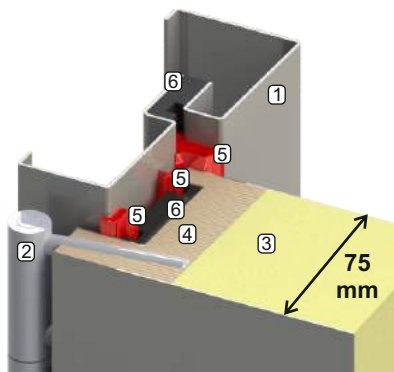
KMT PLUS 75 passive
